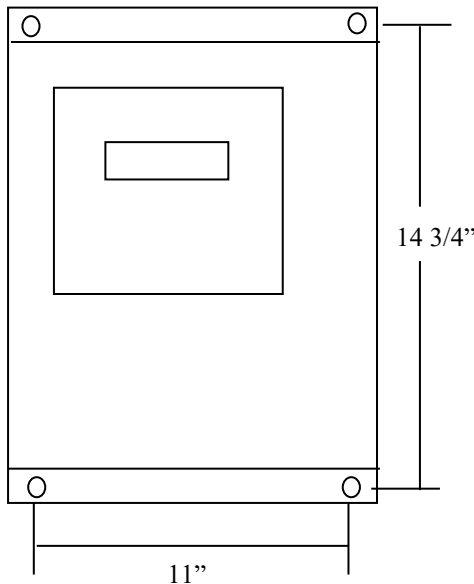
Figure 2 - Mounting Dimensions
