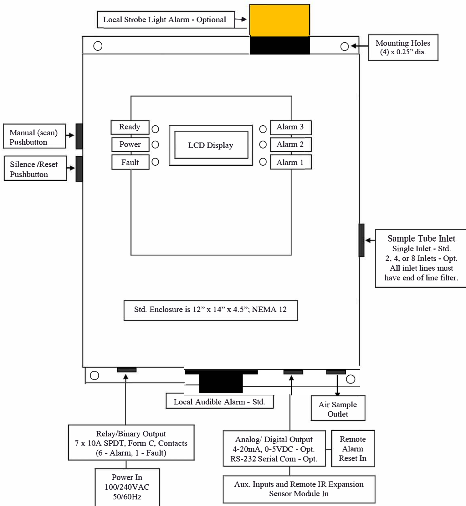
Figure 4 - BLACK BOX Layout Drawing
